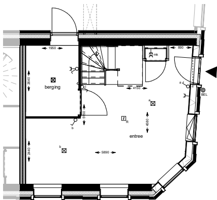
begane grond 1: 50
