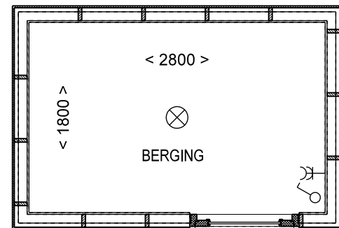
BERGING KAVEL 34, 37, 38
