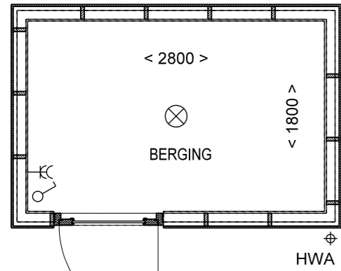
BERGING KAVEL 67
